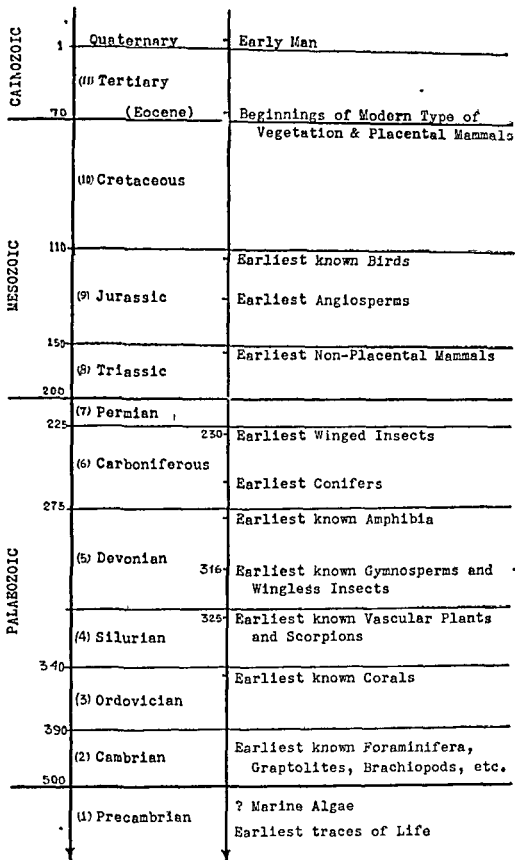
Fig. 4 - The Standard Stratigraphical Scale (simplified from Zeuner, "Dating the Past" 1946). The numbers without brackets represent the approximate ages of the strata in millions of years. Not drawn to scale.
